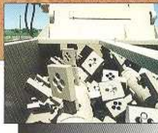
ADJUSTABLE/REVERSIBLE PADDLES: All Pugmill paddles are standard Ni-Hard wear resistant steel. The paddles are adjustable to six (6) positions on the arms to increase retention time and improve mixtures as well as increasing wear life.
