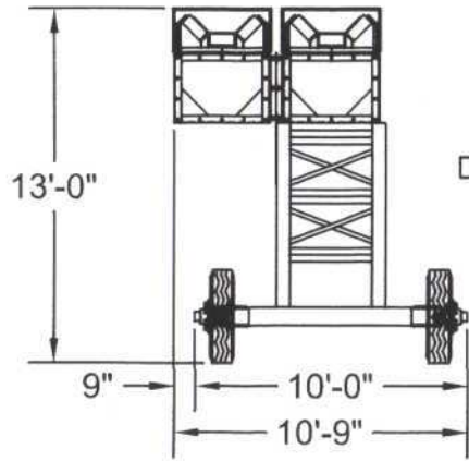
Section A-A: Single Wheel Approximate Weight: 17,600 lbs
