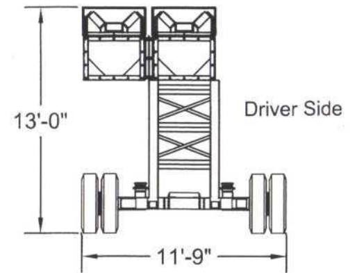
Section A-A: Dual Wheel - Air Brake Approximate Weight: 18,100 lbs Approximate Weight w/ Diesel Module: 20,200 lbs
